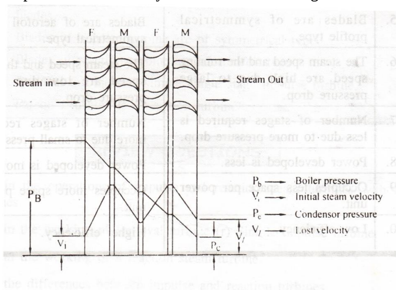
Fig. 26.4 Pressure Velocity Diagram of a Reaction Turbine
