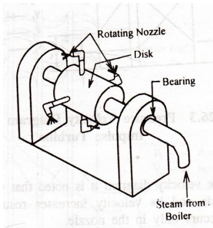
Fig. 26.2 Reaction Turbine
