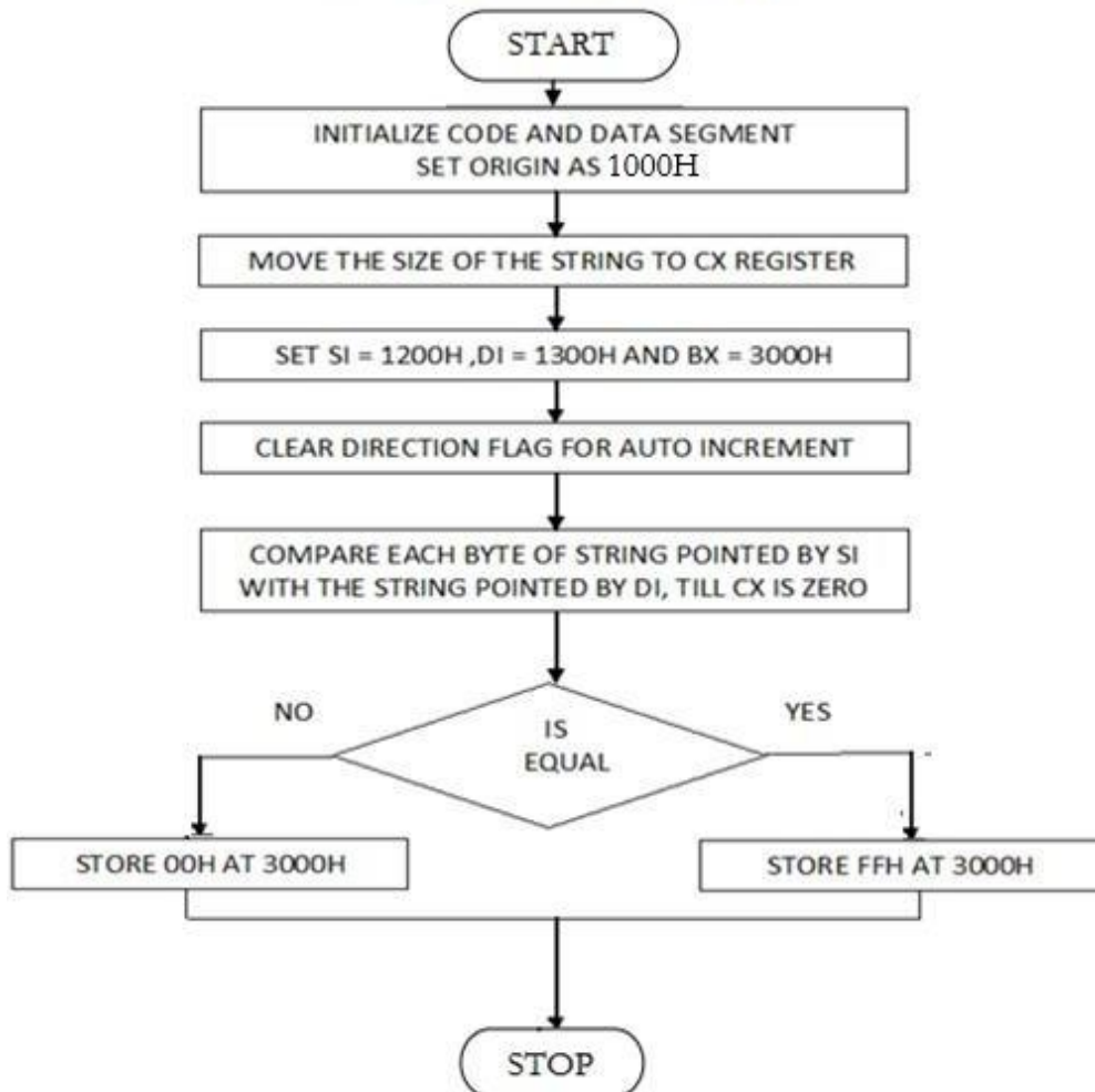
Flowchart for Comparing two Strings
